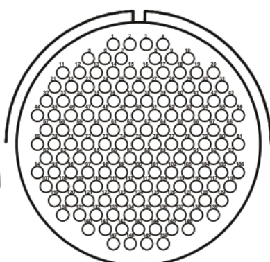
150 pin / size 40
