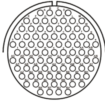
85 pin / size 40
