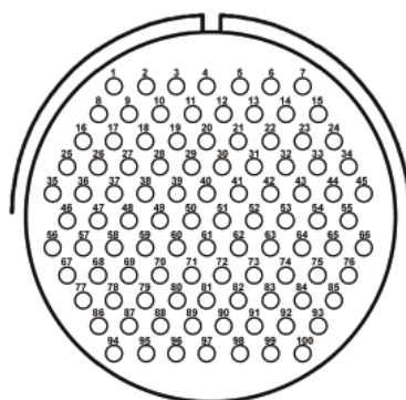
100 pin / size 40
