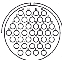
37 pin / size 28
