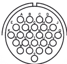
25 pin / size 24
