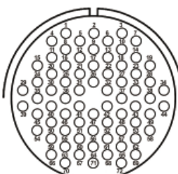
72 pin / size 28
