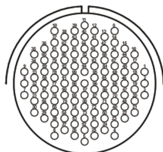
101 pin / size 32
