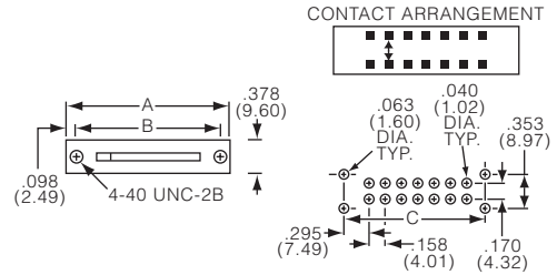
CONTACT ARRANGEMENT
